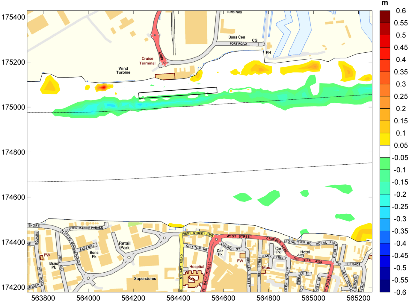
Figure 17.24: Essex Project Site Baseline predicted patterns for erosion and deposition.
